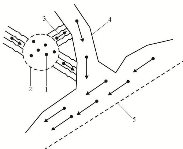
1 – methane molecule; 2 – micropore wall; 3 – supermicropores and mesopores, where Volmer diffusion takes place; 4 – interlayer space; 5 – macrocrack
